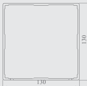
Post profile
