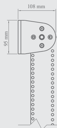
Wall/ceiling bracket dimensions
