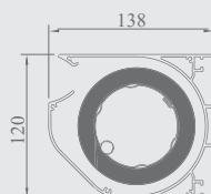
Cassette cross-section
