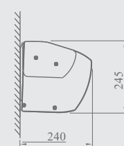
Wall installation
