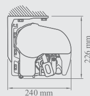
Ceiling installation
