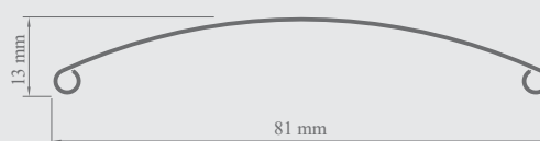
Slat cross-section
