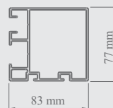
Guide rail cross-section
