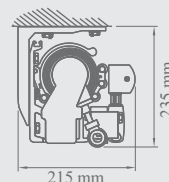
Ceiling installation
