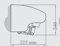
Wall installation - option with hood
