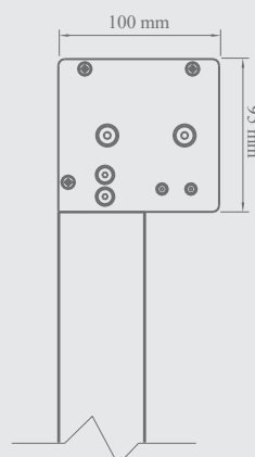
Cassette dimensions
