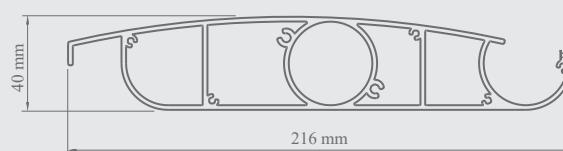
Blade cross-section
