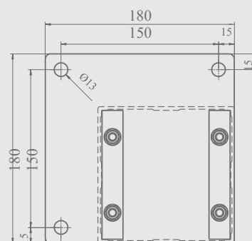
Feet
