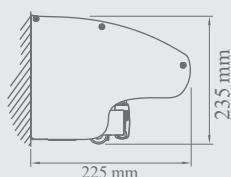
Wall installation - option with hood
