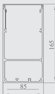
Beam profile
