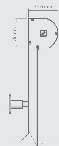
Cassette dimensions
