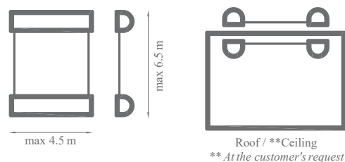
Group installation
