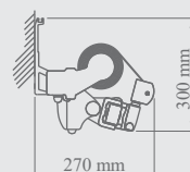
Wall installation
