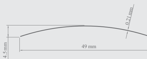
Slat cross-section
