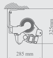
Ceiling installation
