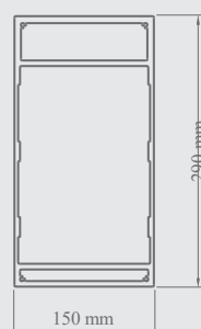
Beam cross-section
